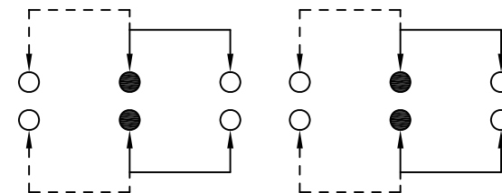
SCHEMATIC (NON-SHORTING)
